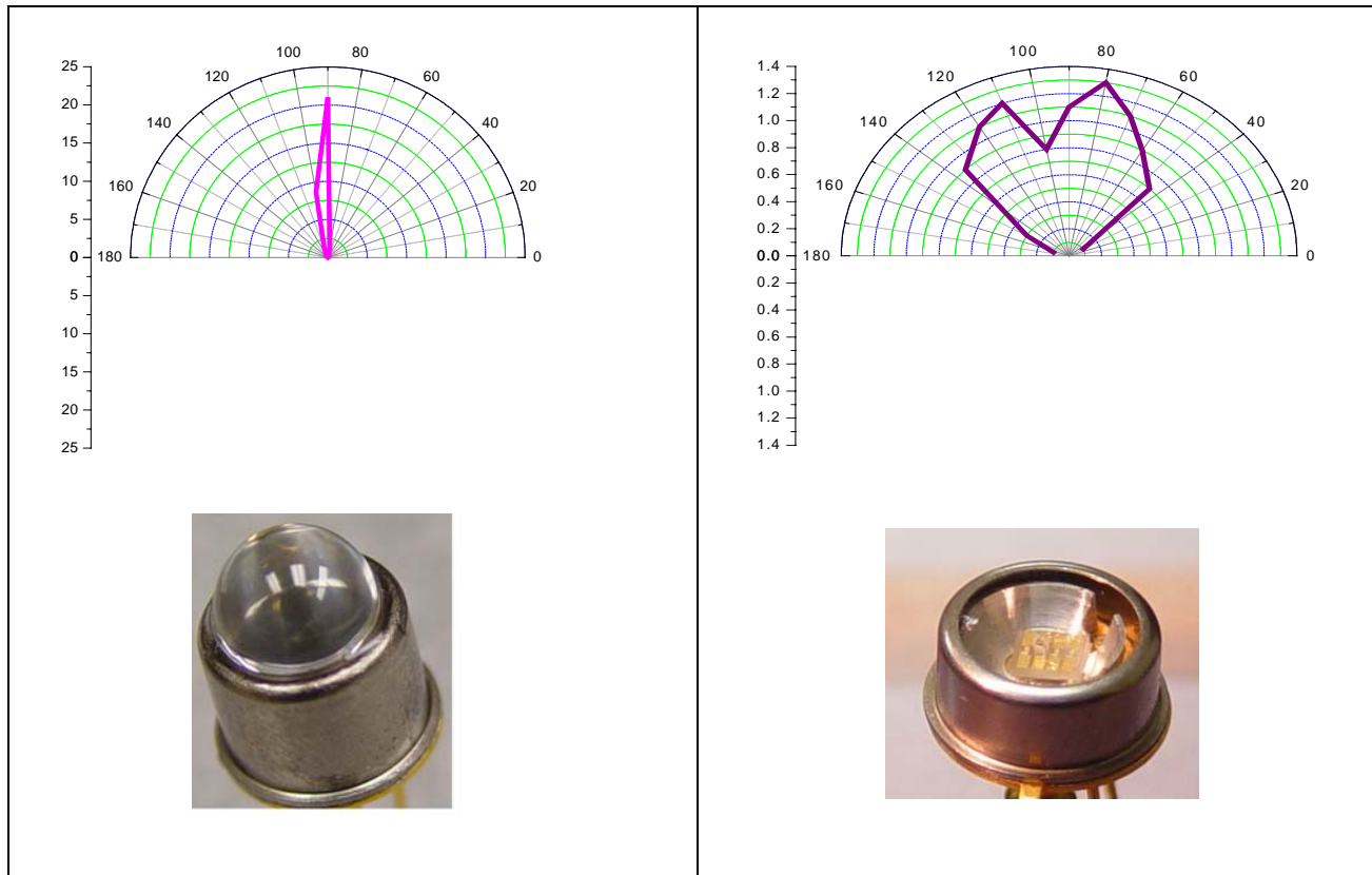
Typical angular diagrams (not the datasheet limits)
