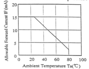
Allowable Forward Current vs. Ambient Temperature
