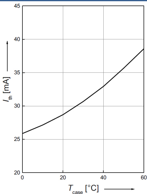
Threshold Current
