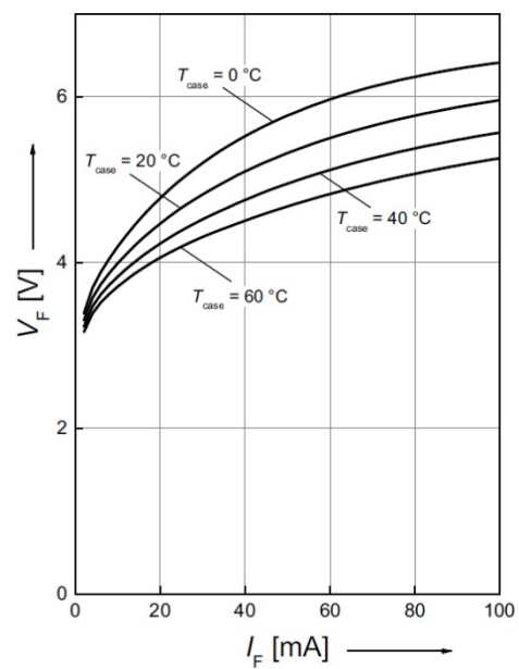
Operating Voltage
