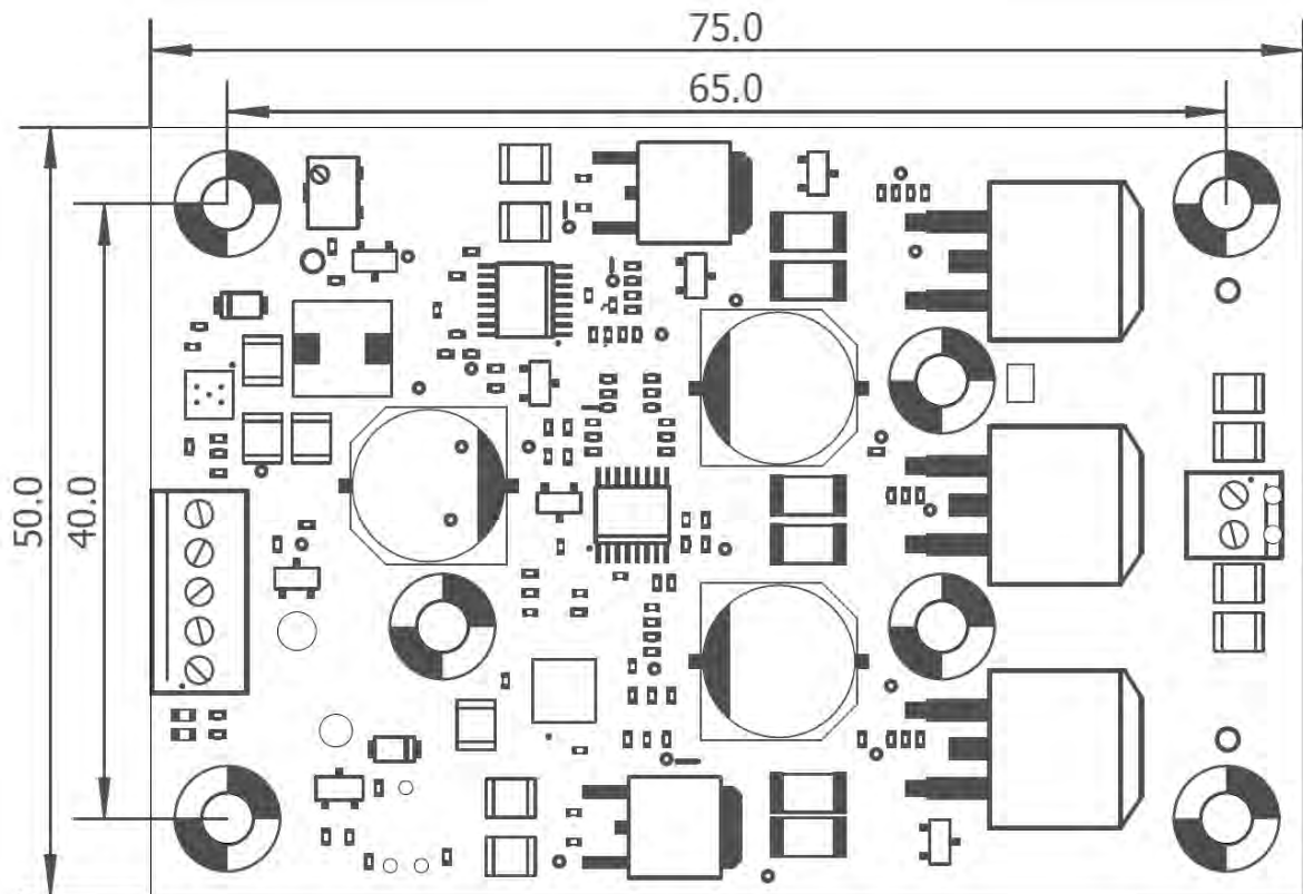
Fig. 12: PCB dimensions
