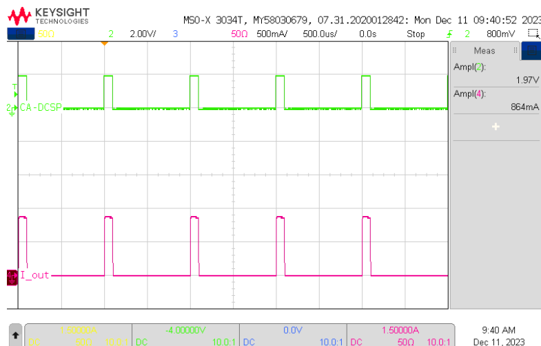
Fig. 9: Pulsed operation
