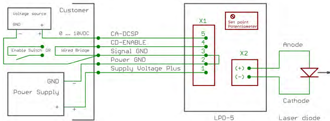
Fig. 6: Wiring diagram with LDP-5023 operating in CW mode.
