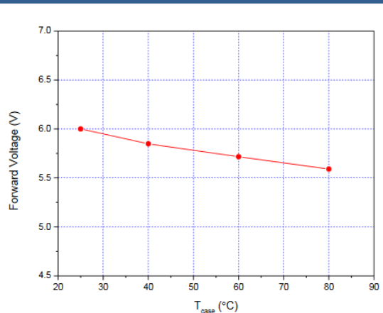
Forward Voltage vs. Case Temperature*
