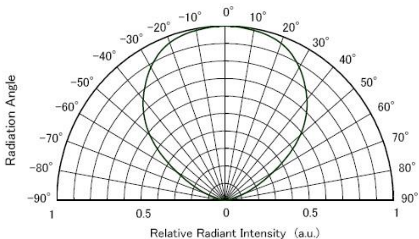
Directivity
