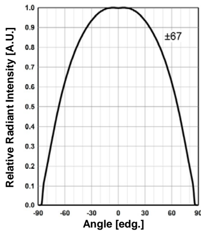
Radiation Characteristics
