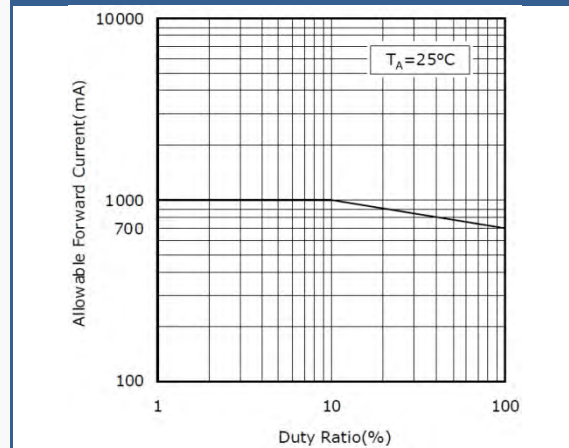
Duty Ratio vs. Allowable Forward Current
